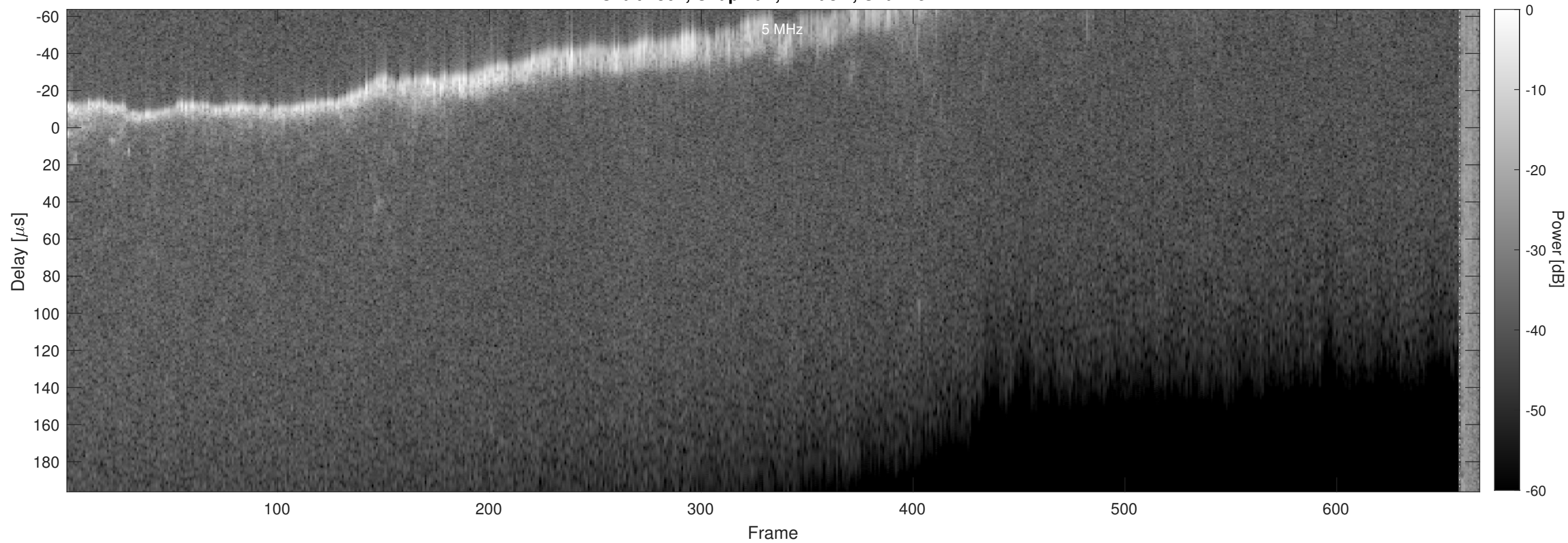
Orbit 7362, Chapman, Window, Channel 2
