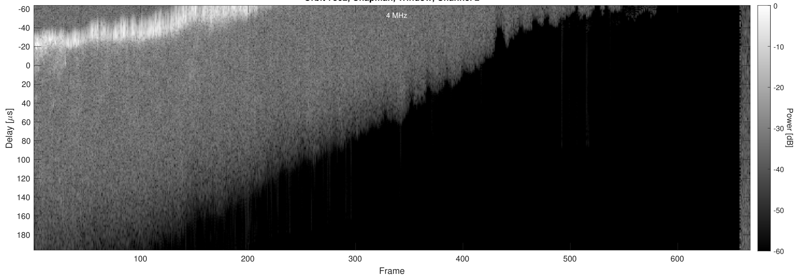
Orbit 7362, Chapman, Window, Channel 2
