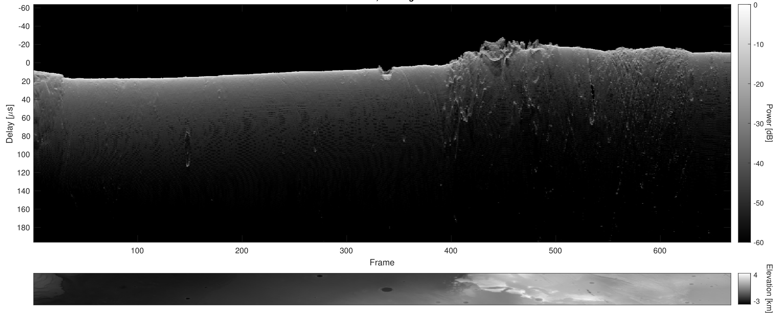
Orbit 7362, Cluttergram
