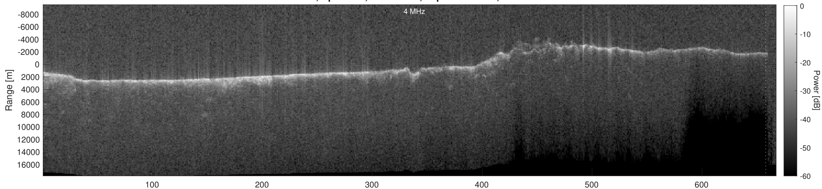
Orbit 7362, Depth-Corrected Cluttergram
