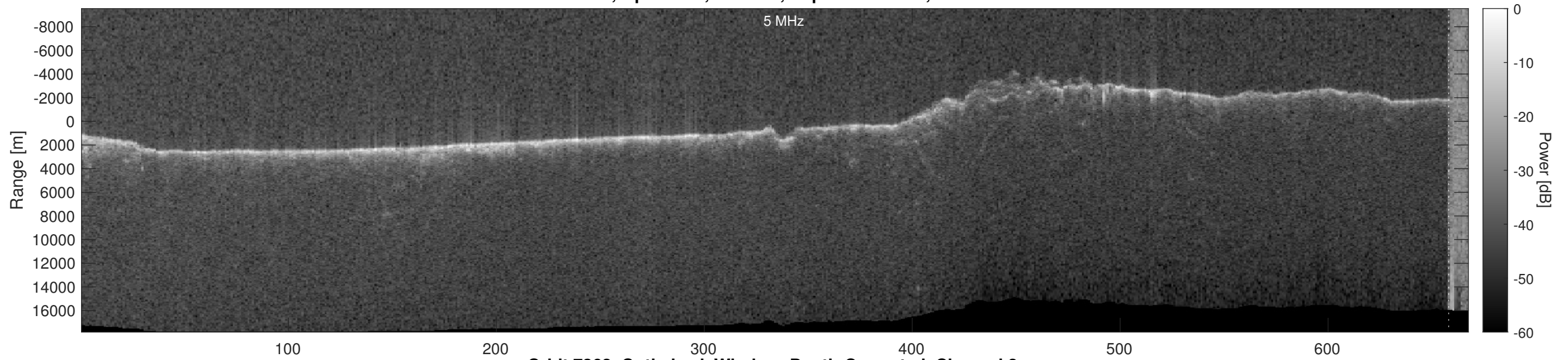
Orbit 7362, Optimized, Window, Depth-Corrected, Channel 2
