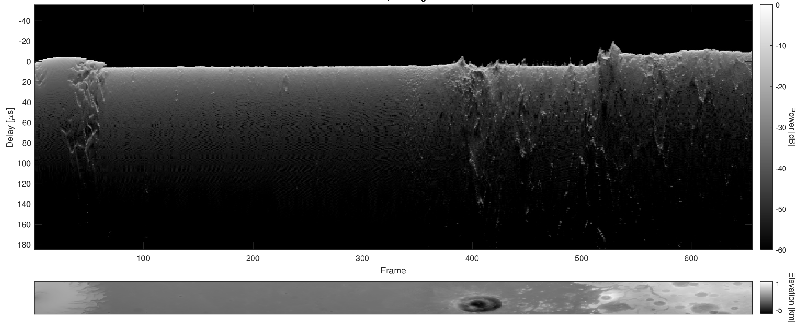
Orbit 7368, Cluttergram
