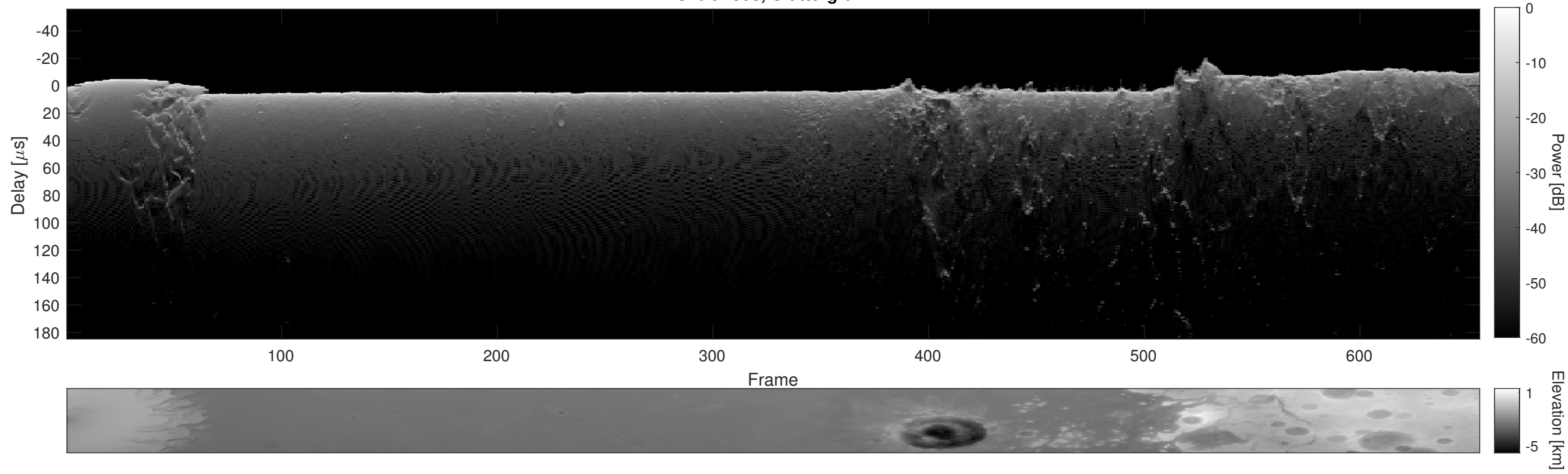
Orbit 7368, Cluttergram
