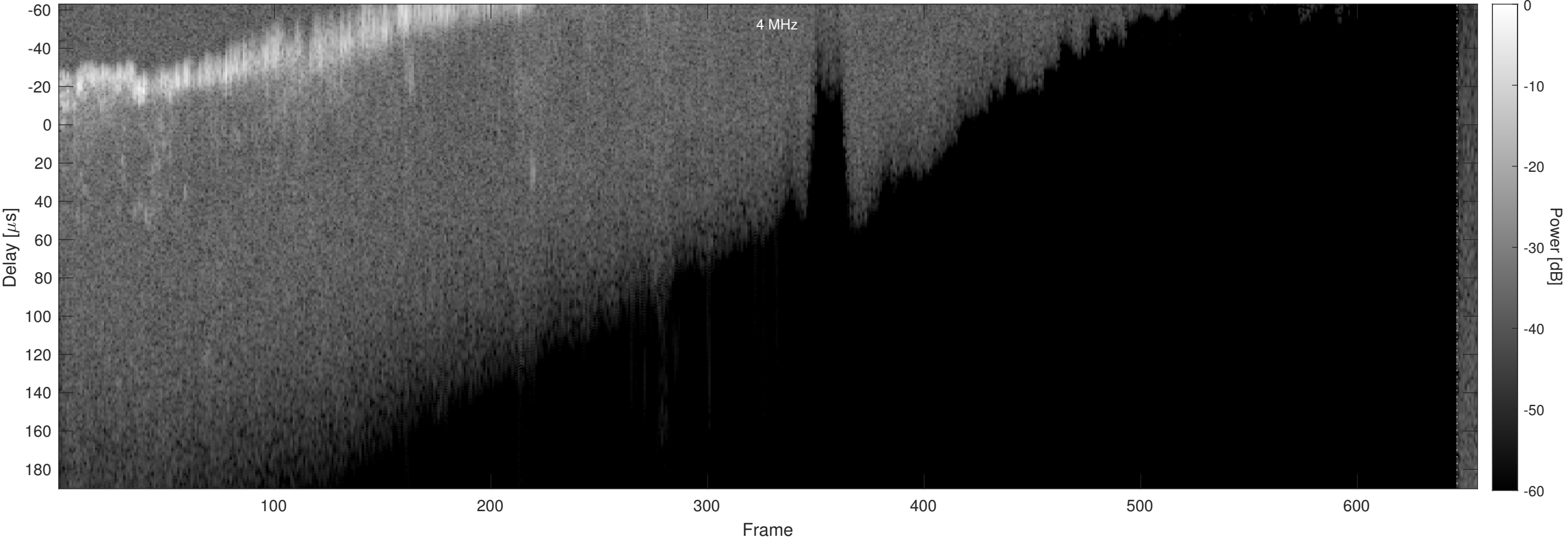
Orbit 7369, Chapman, Window, Channel 2
