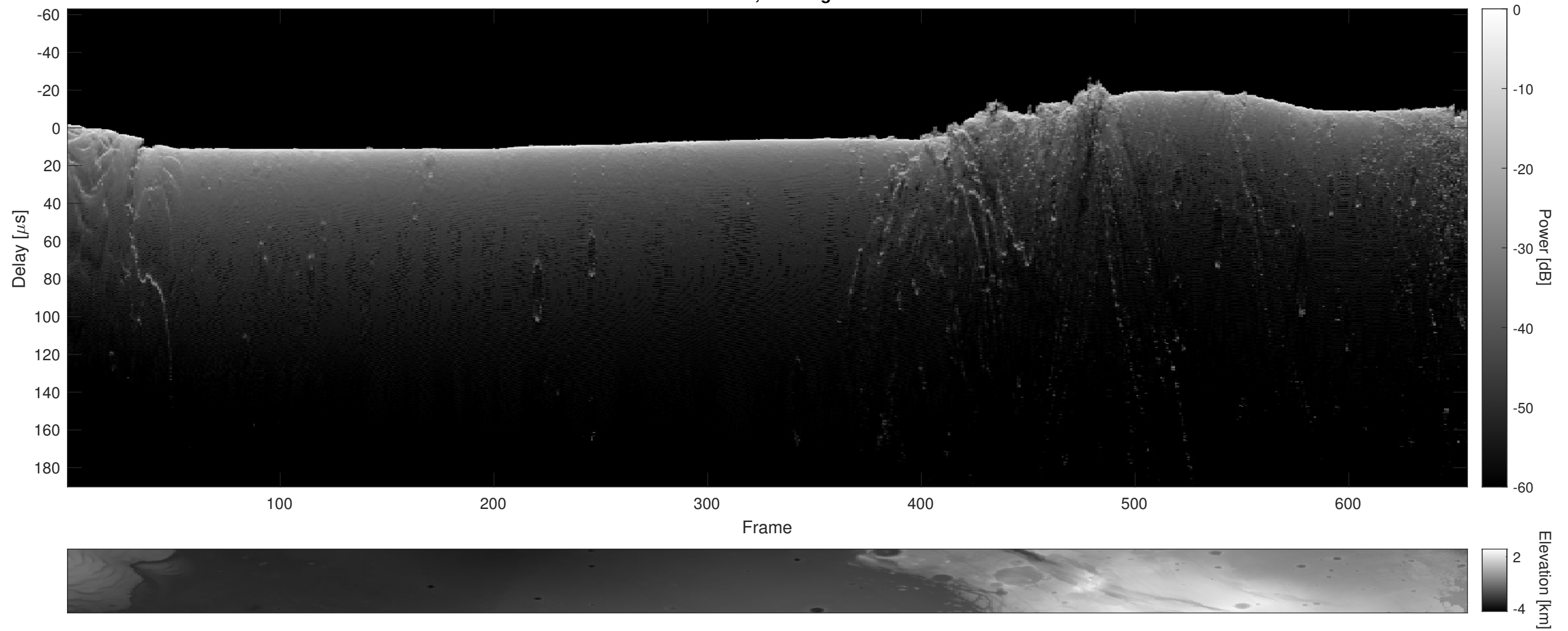
Orbit 7369, Cluttergram
