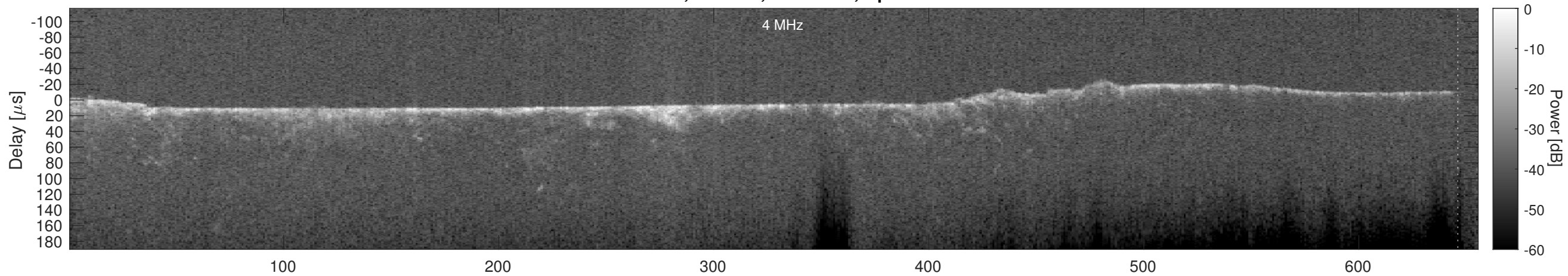
Orbit 7369, Cluttergram
