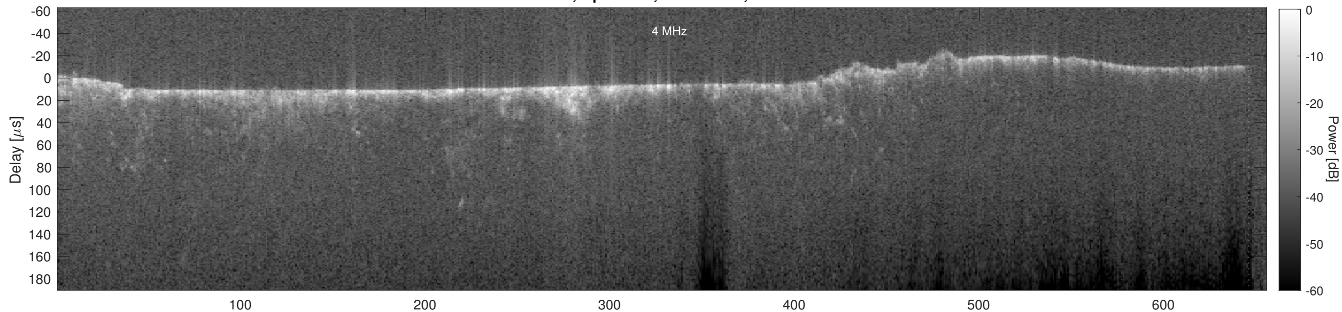
Orbit 7369, Cluttergram
