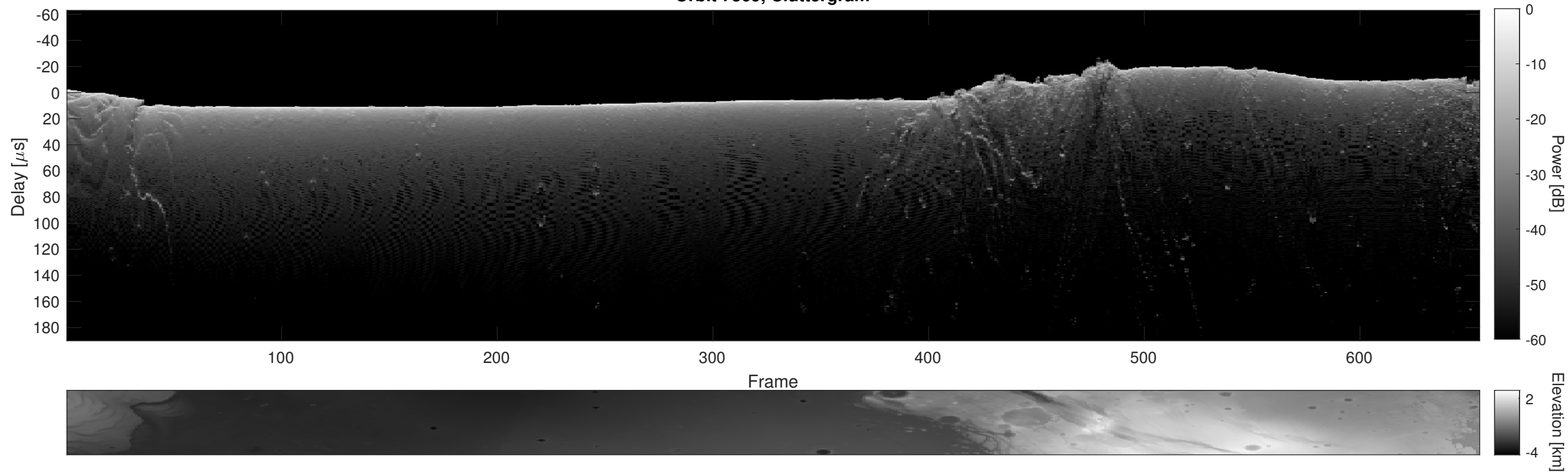
Orbit 7369, Cluttergram
