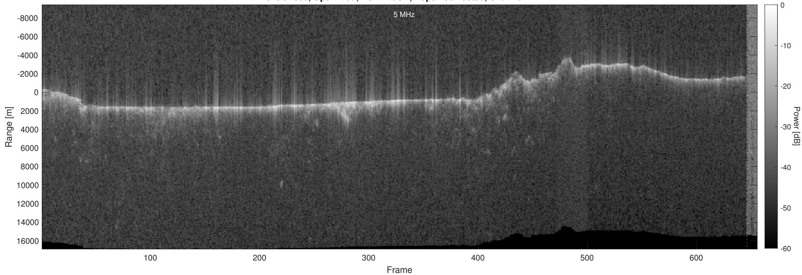
Orbit 7369, Optimized, No Window, Depth-Corrected, Channel 2
