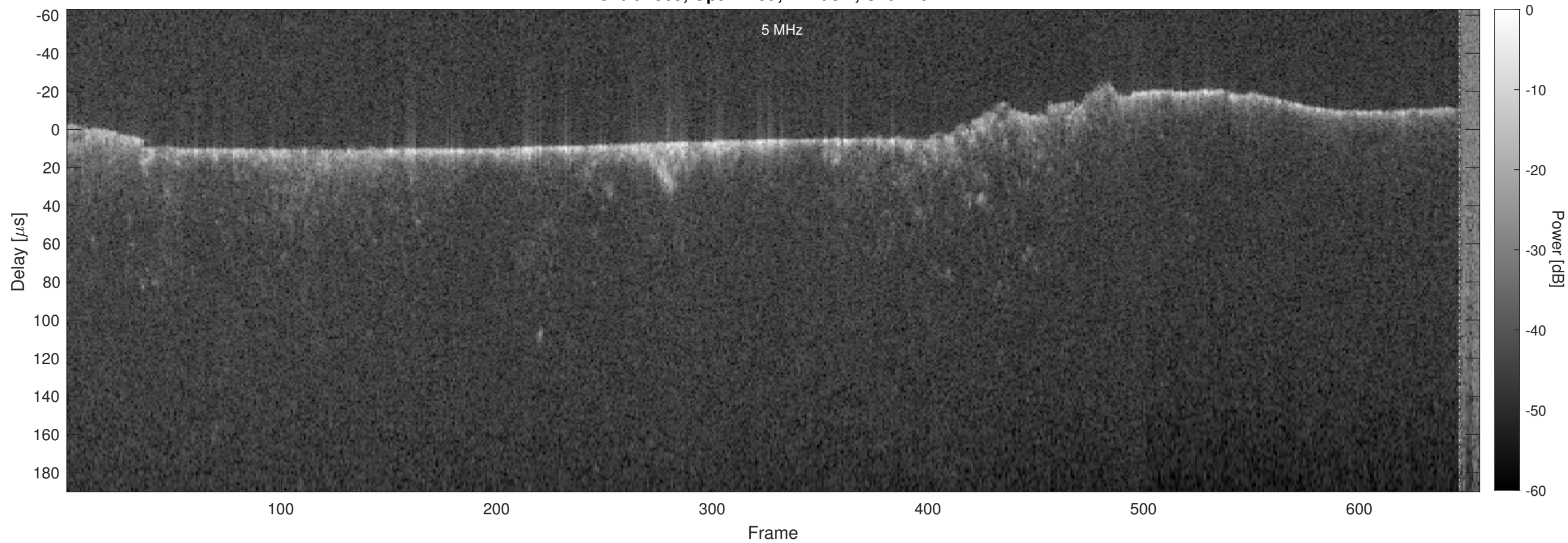
Orbit 7369, Optimized, Window, Channel 2
