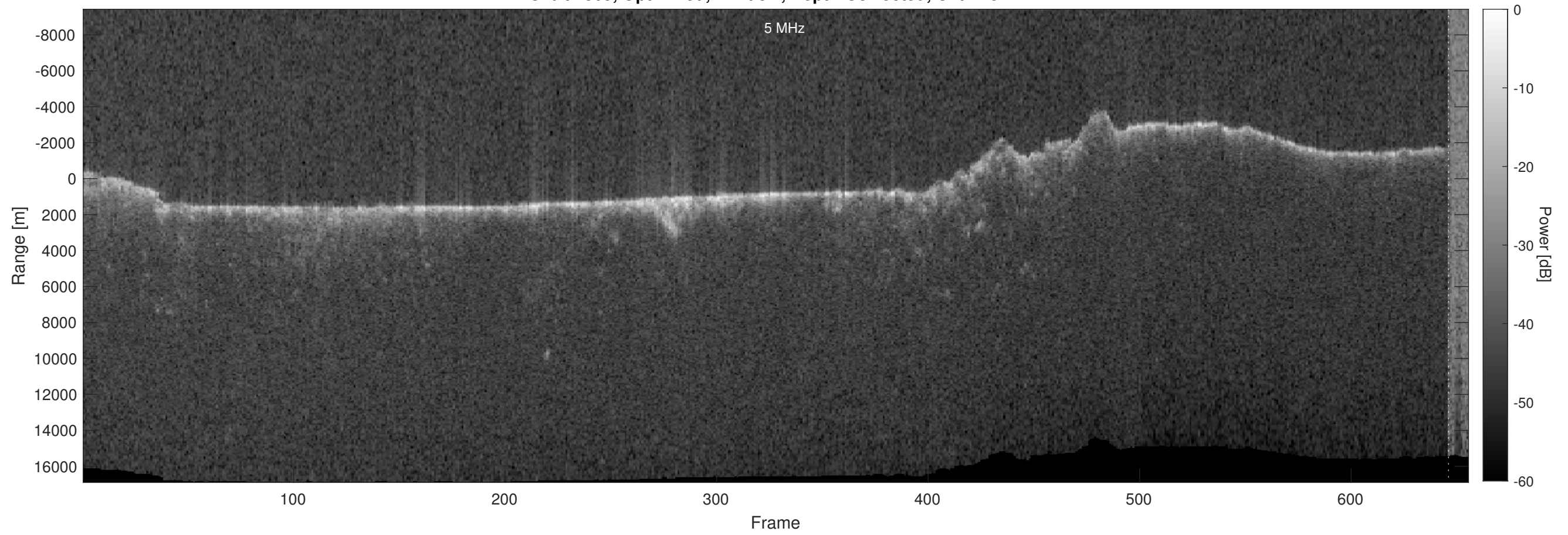
Orbit 7369, Optimized, Window, Depth-Corrected, Channel 2
