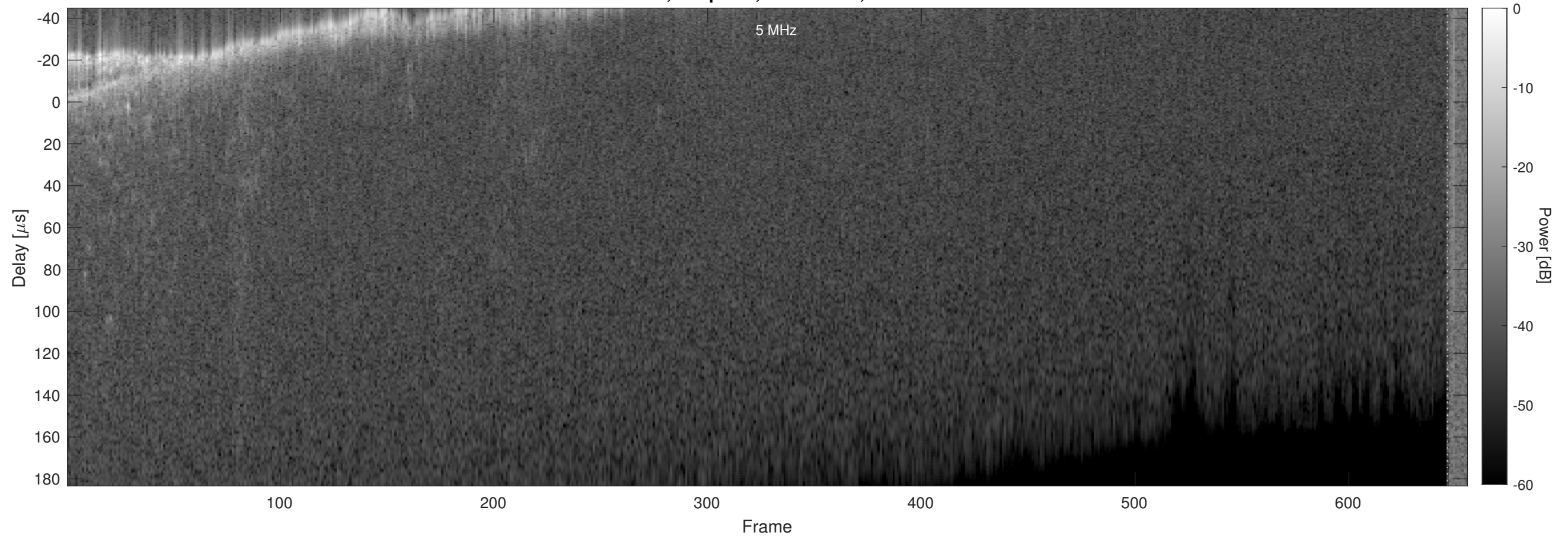
Orbit 7371, Chapman, No Window, Channel 2
