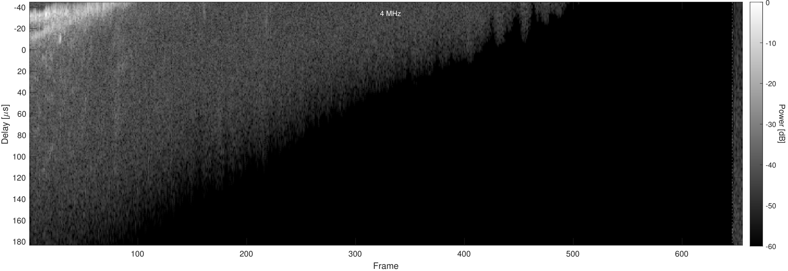
Orbit 7371, Chapman, Window, Channel 2
