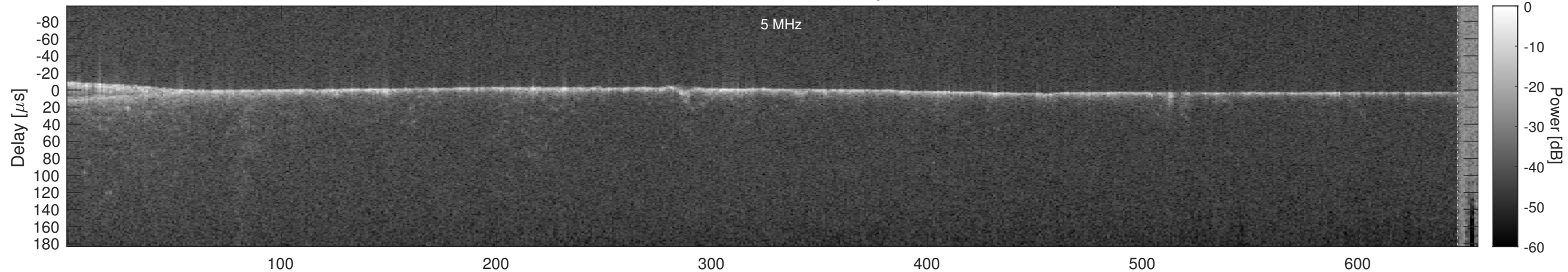
Orbit 7371, Cluttergram
