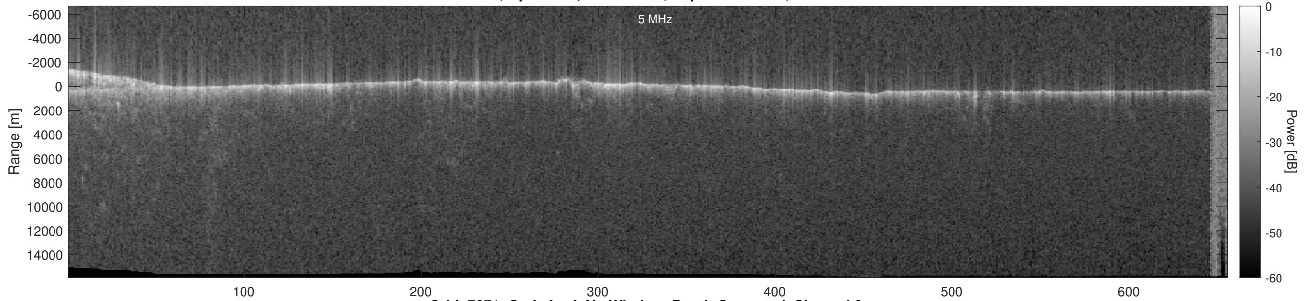
Orbit 7371, Optimized, No Window, Depth-Corrected, Channel 2
