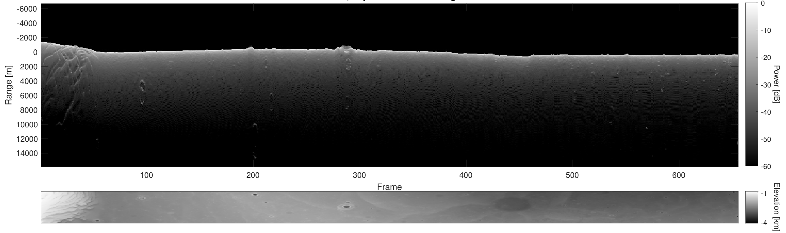
Orbit 7371, Depth-Corrected Cluttergram
