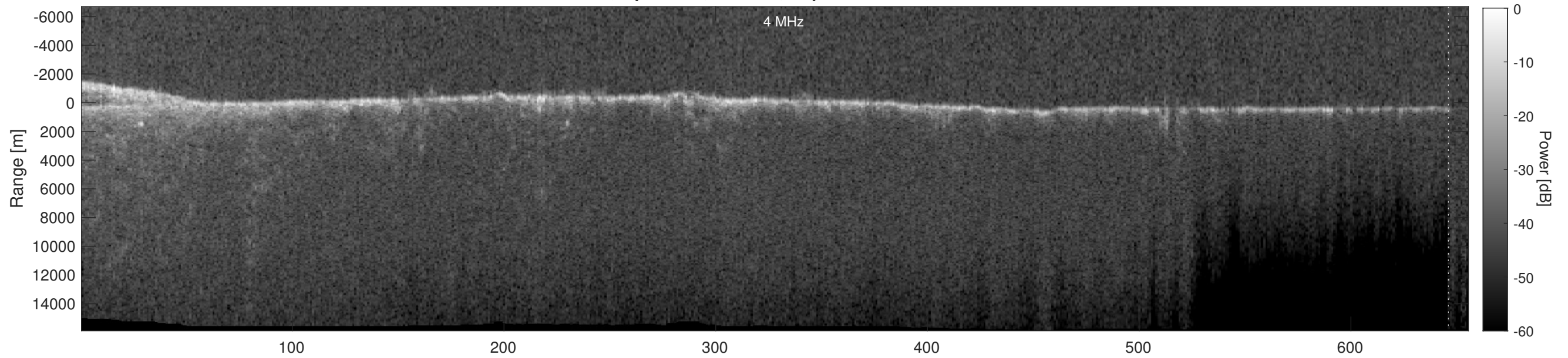
Orbit 7371, Depth-Corrected Cluttergram
