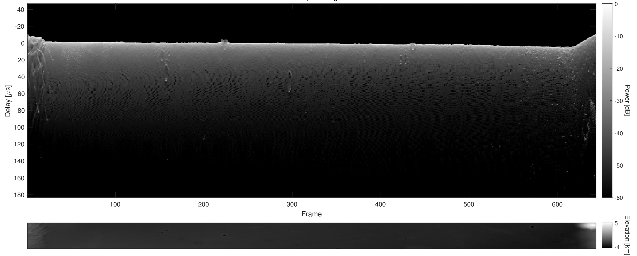
Orbit 7374, Cluttergram
