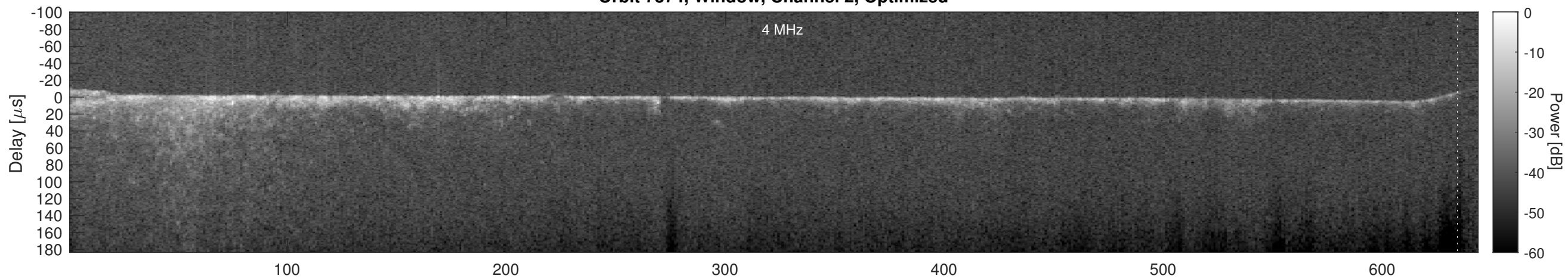
Orbit 7374, Cluttergram
