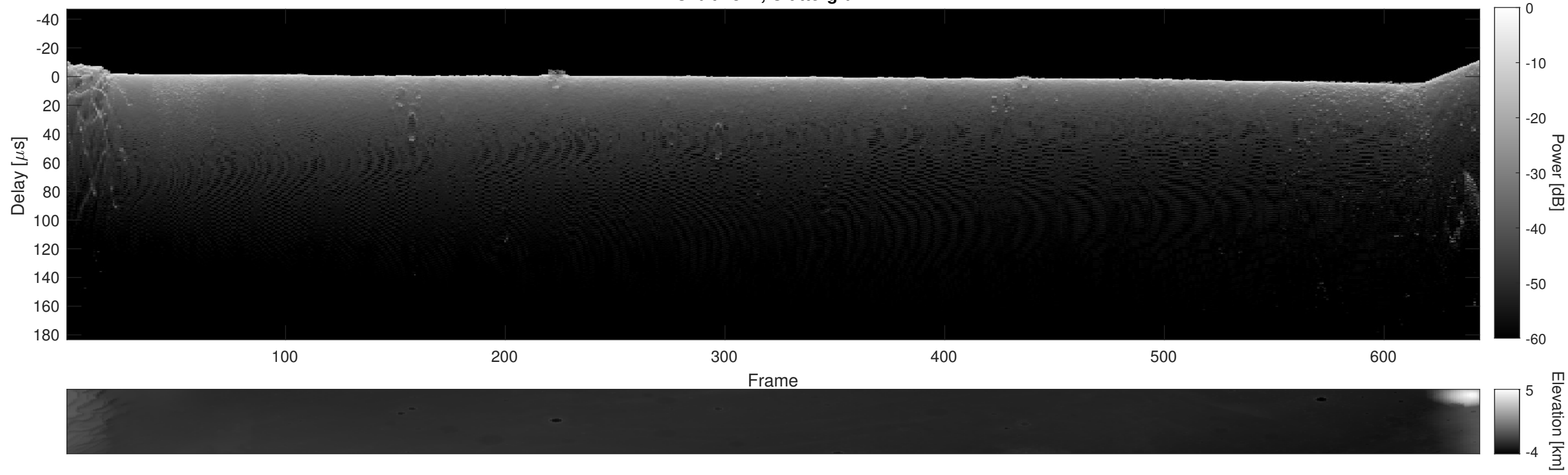
Orbit 7374, Cluttergram
