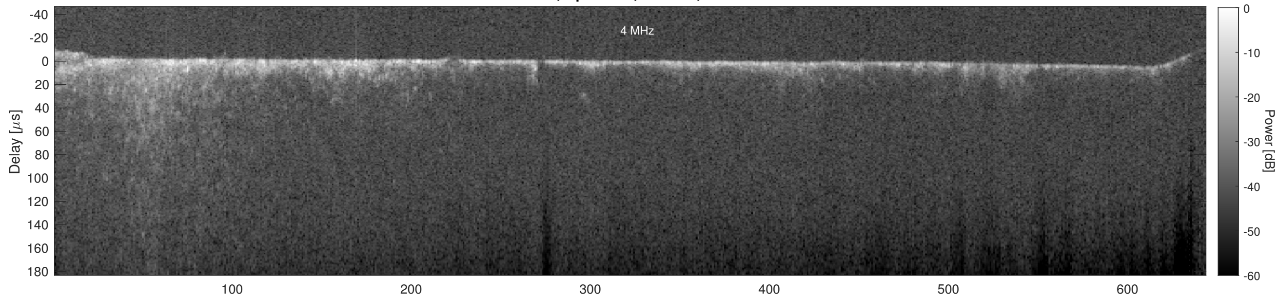
Orbit 7374, Cluttergram
