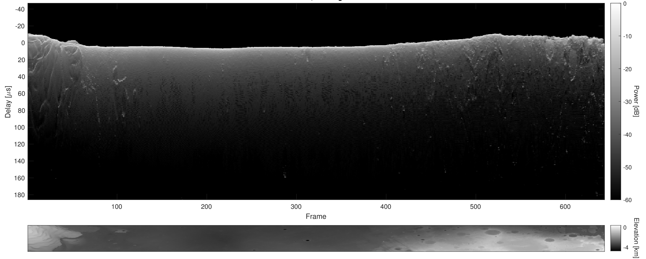
Orbit 7376, Cluttergram
