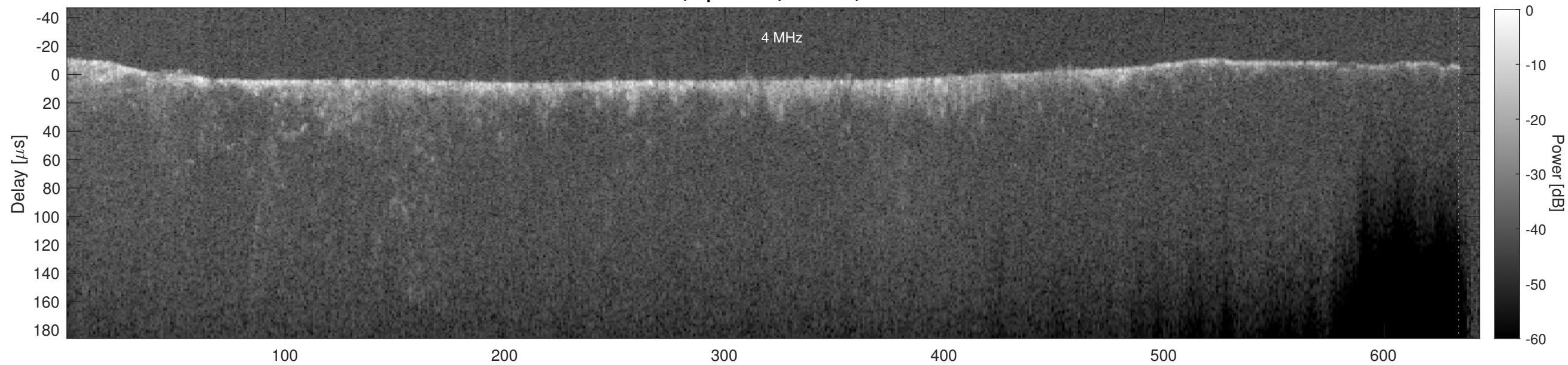
Orbit 7376, Cluttergram
