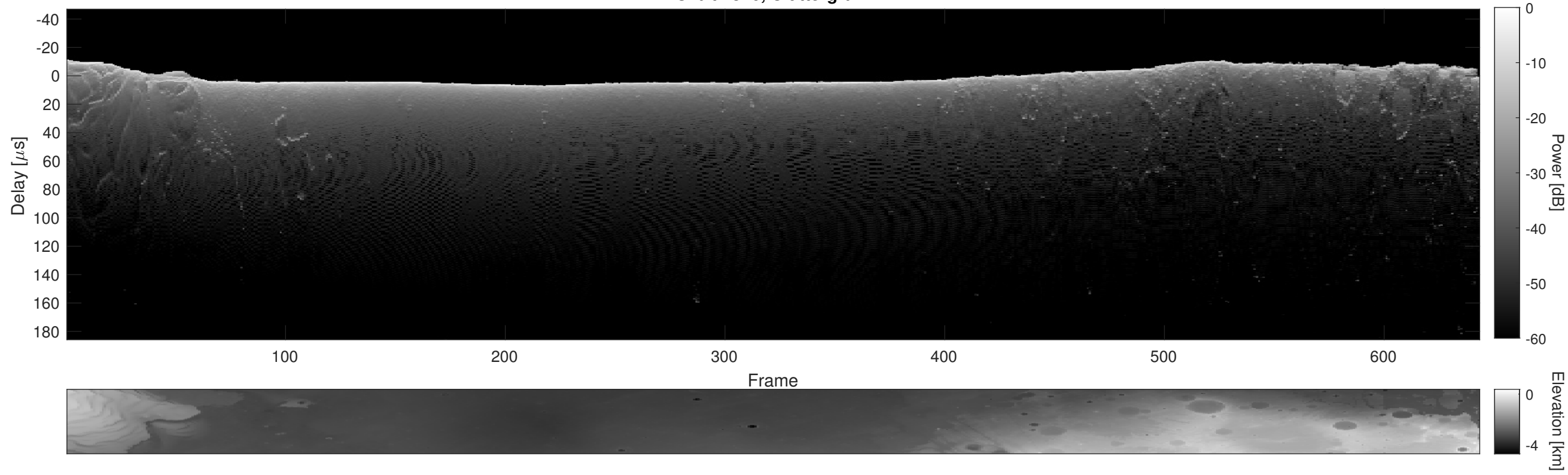
Orbit 7376, Cluttergram
