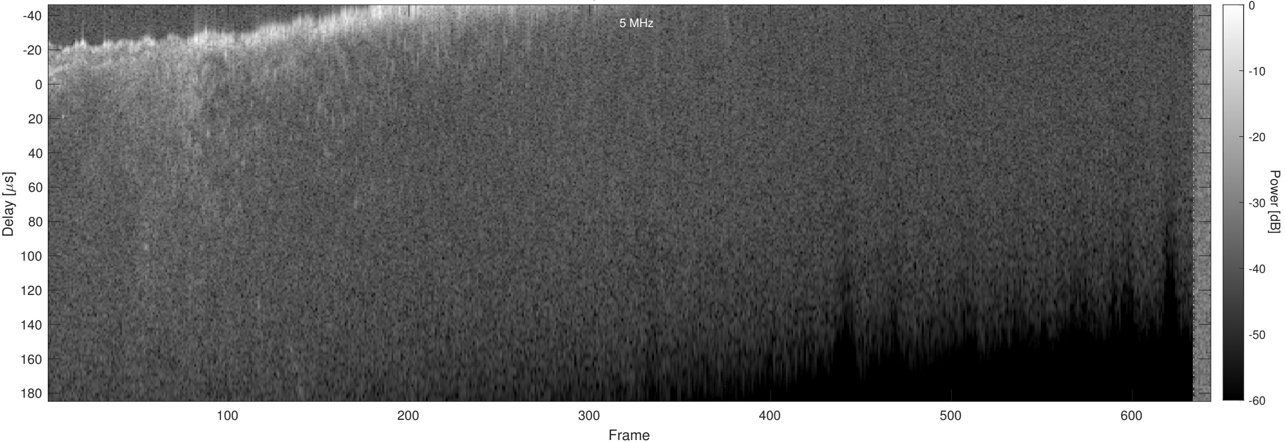
Orbit 7377, Chapman, Window, Channel 2
