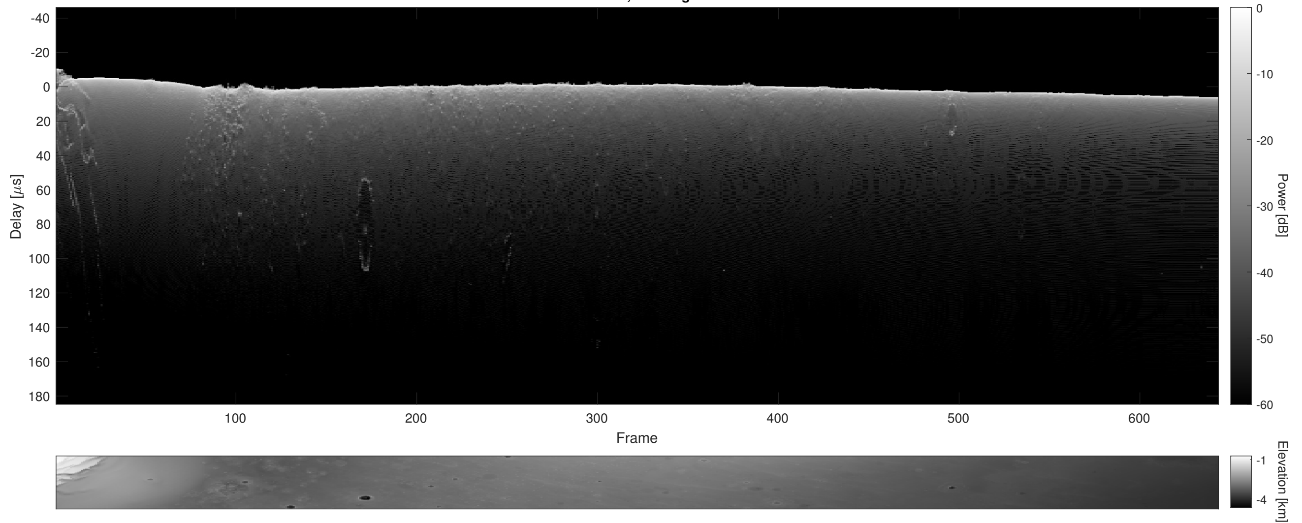
Orbit 7377, Cluttergram
