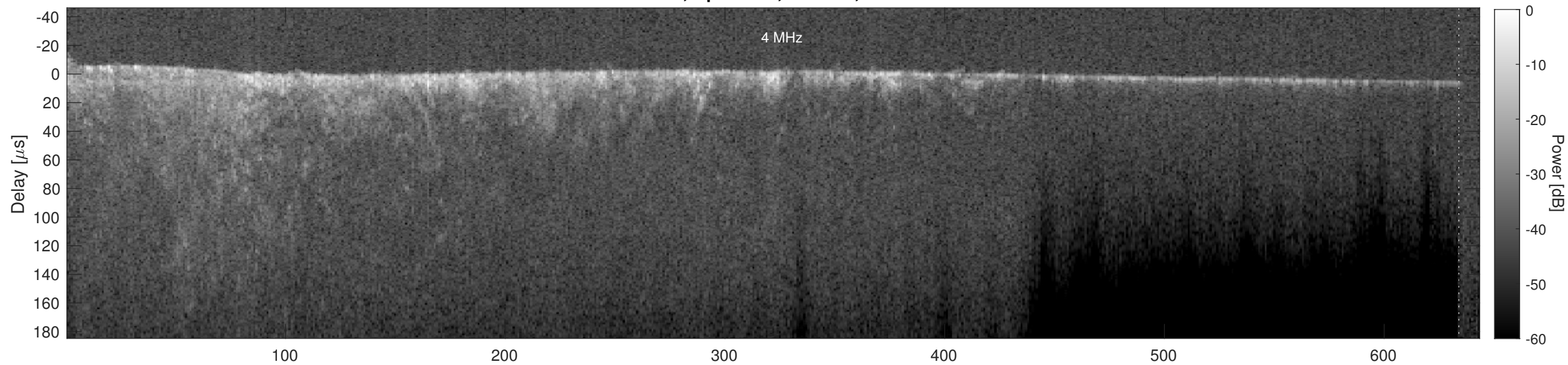
Orbit 7377, Cluttergram
