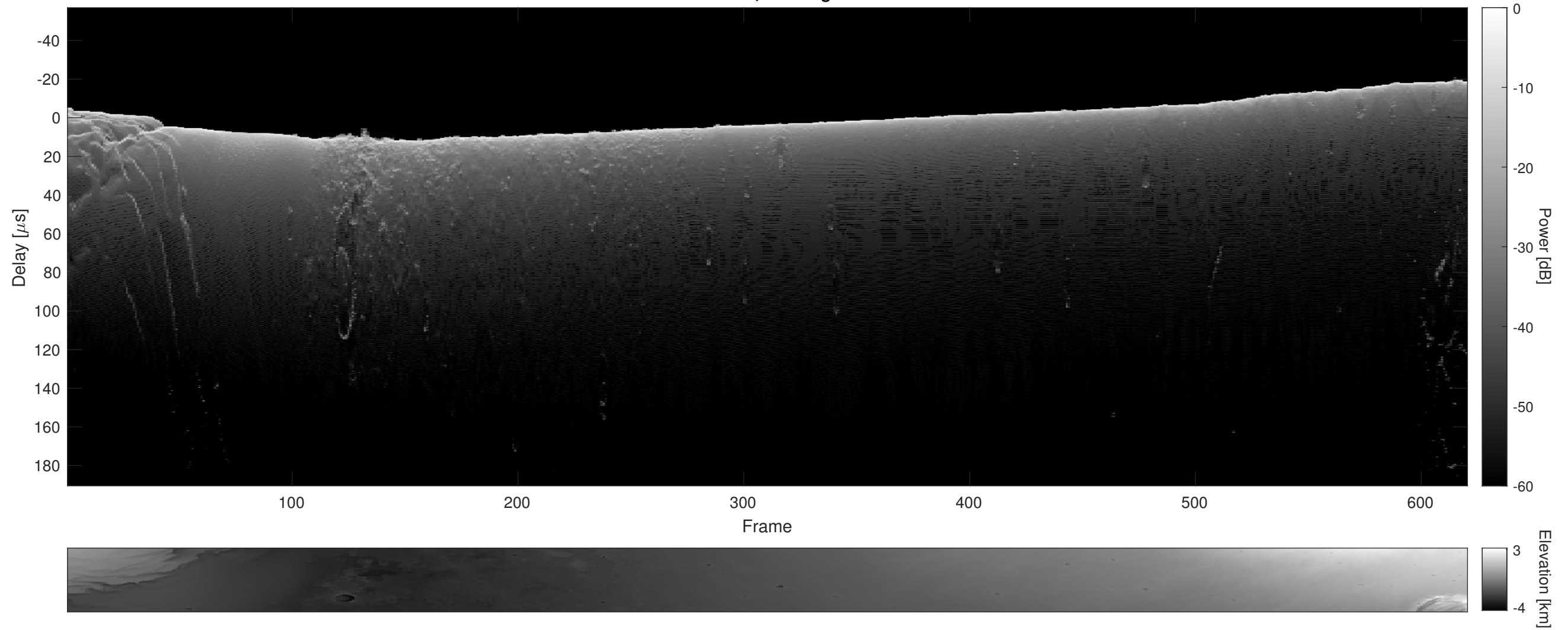
Orbit 7391, Cluttergram
