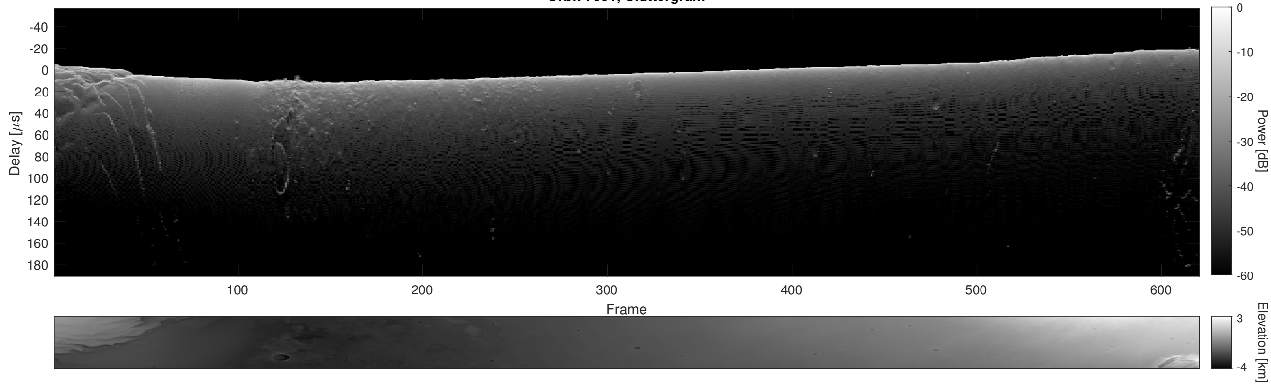
Orbit 7391, Cluttergram
