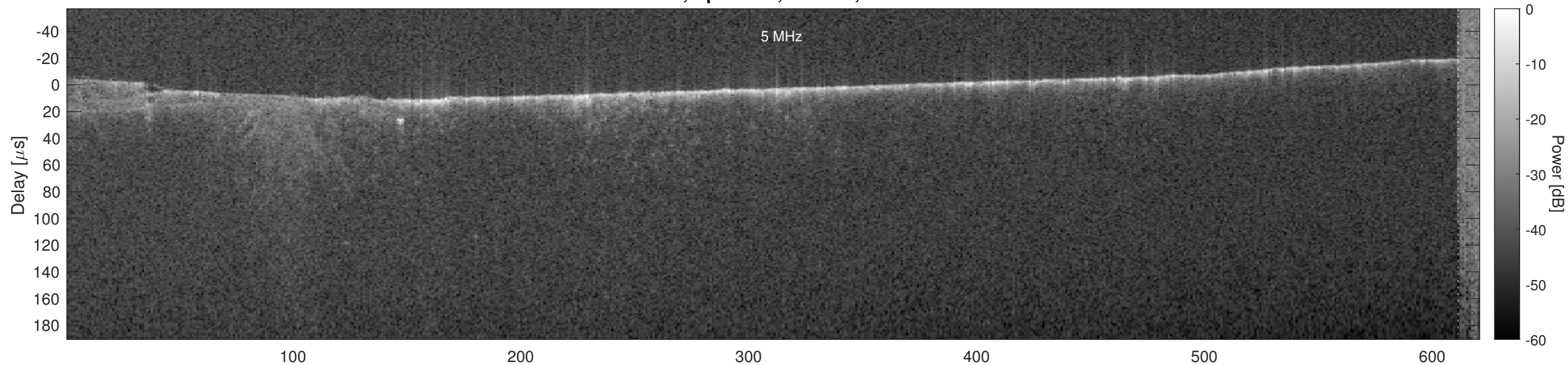
Orbit 7391, Optimized, Window, Channel 2
