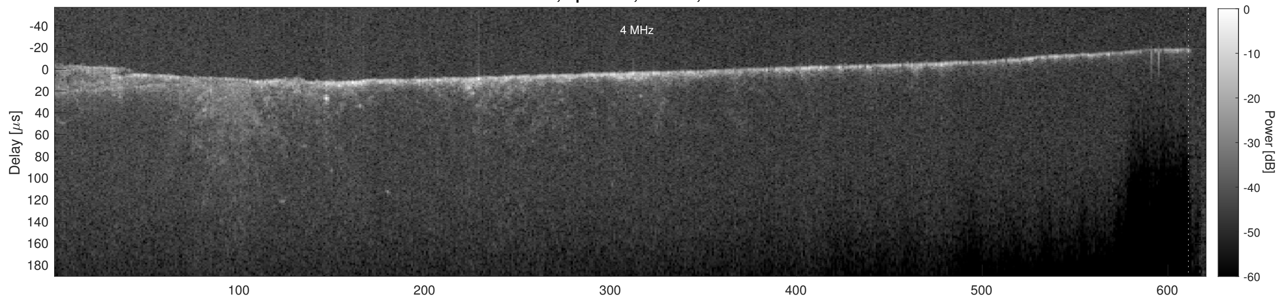
Orbit 7391, Cluttergram
