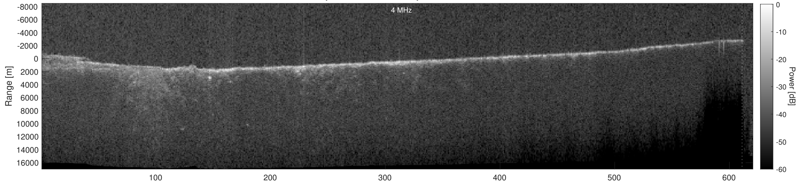
Orbit 7391, Depth-Corrected Cluttergram
