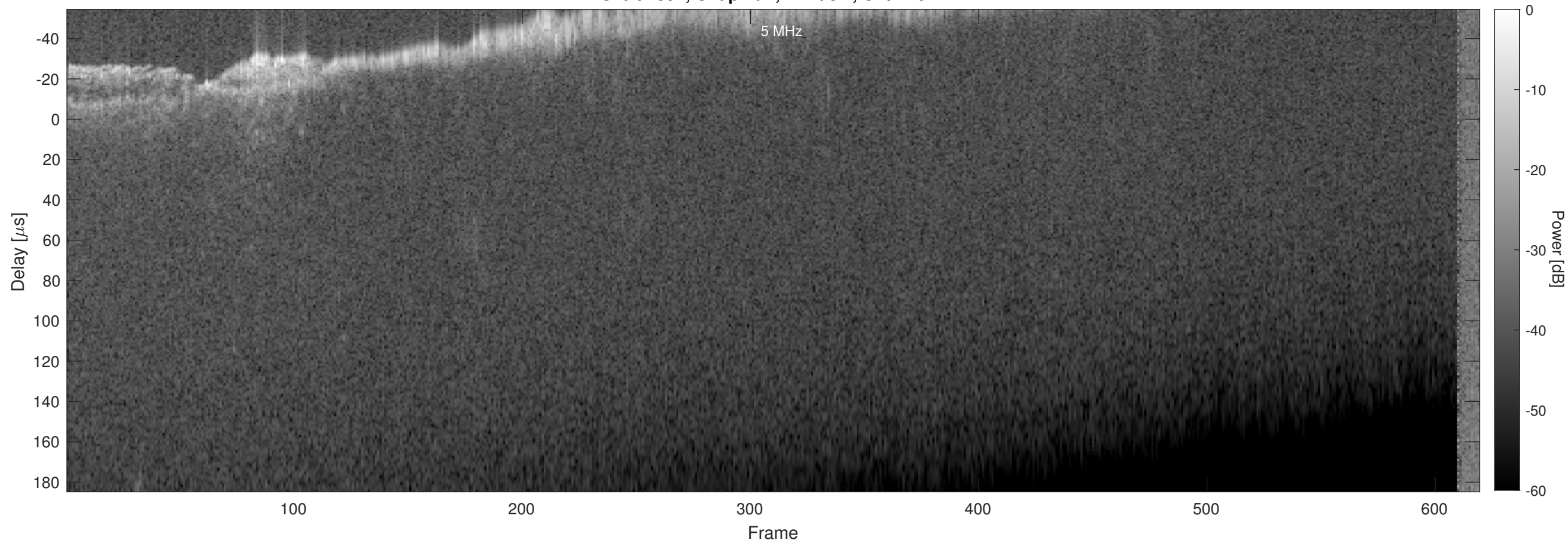
Orbit 7397, Chapman, Window, Channel 2
