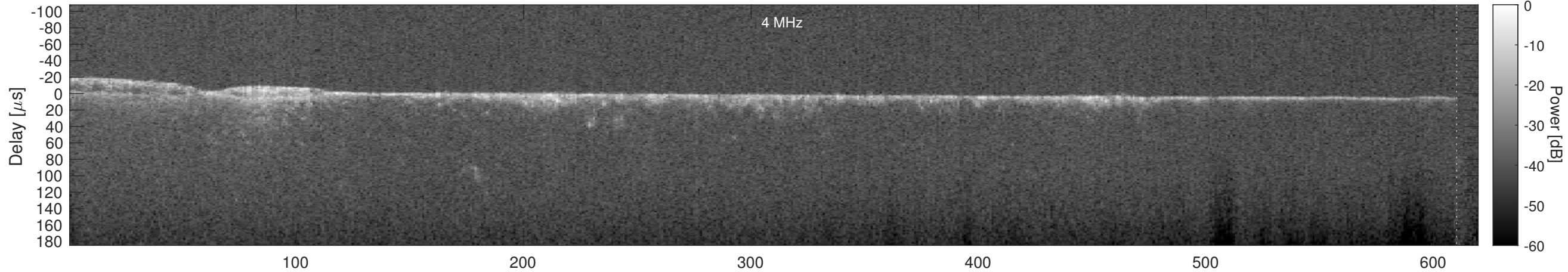
Orbit 7397, Cluttergram
