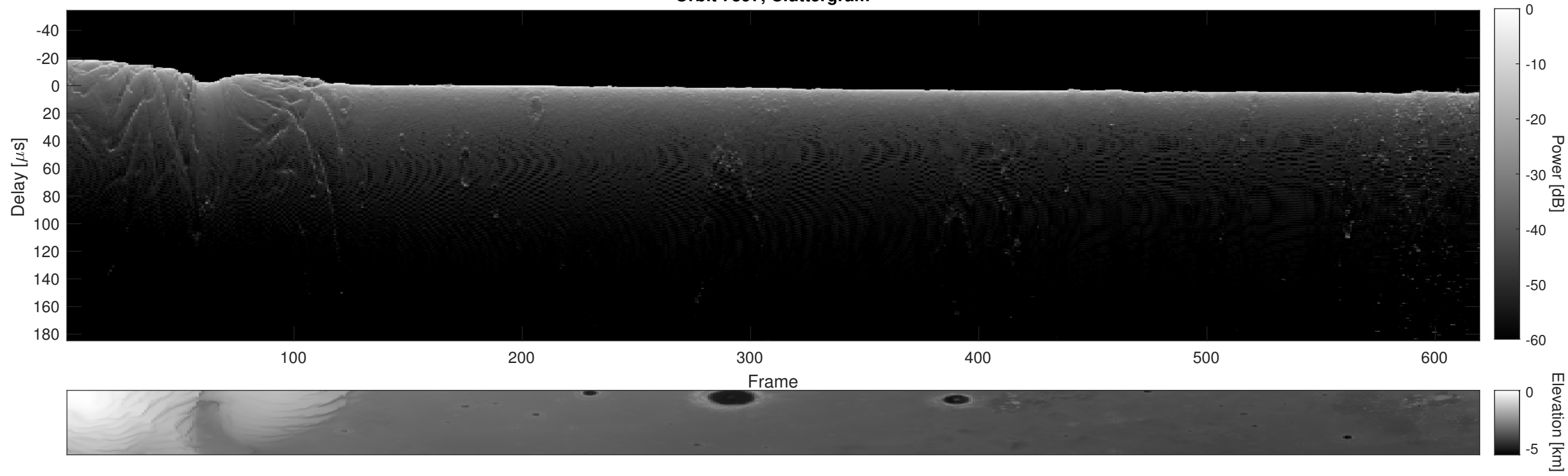
Orbit 7397, Cluttergram
