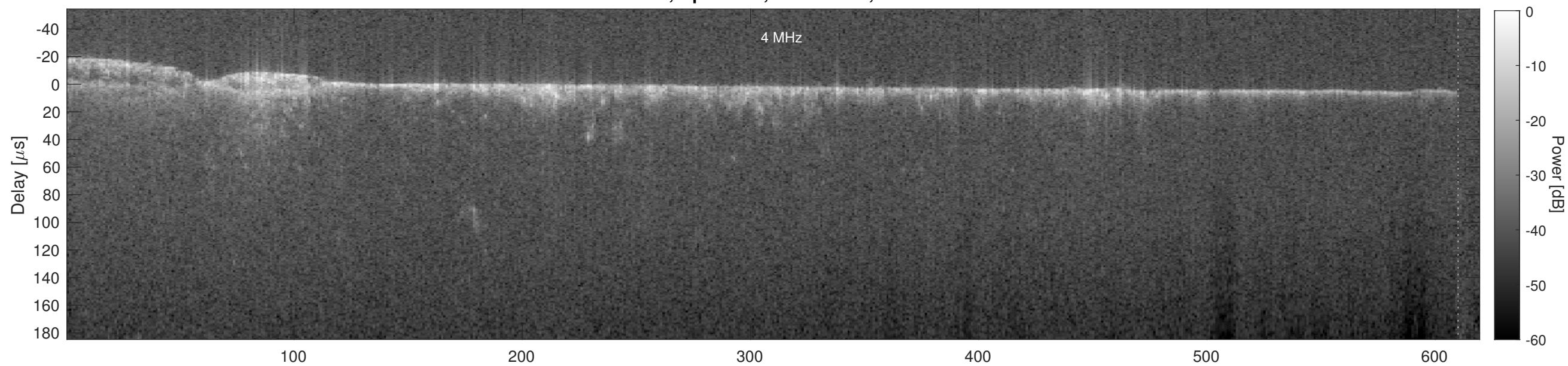
Orbit 7397, Cluttergram
