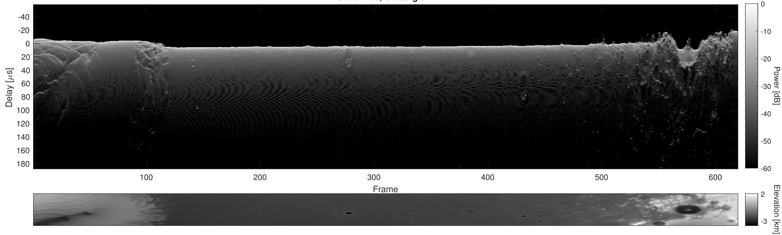
Orbit 7400, Cluttergram
