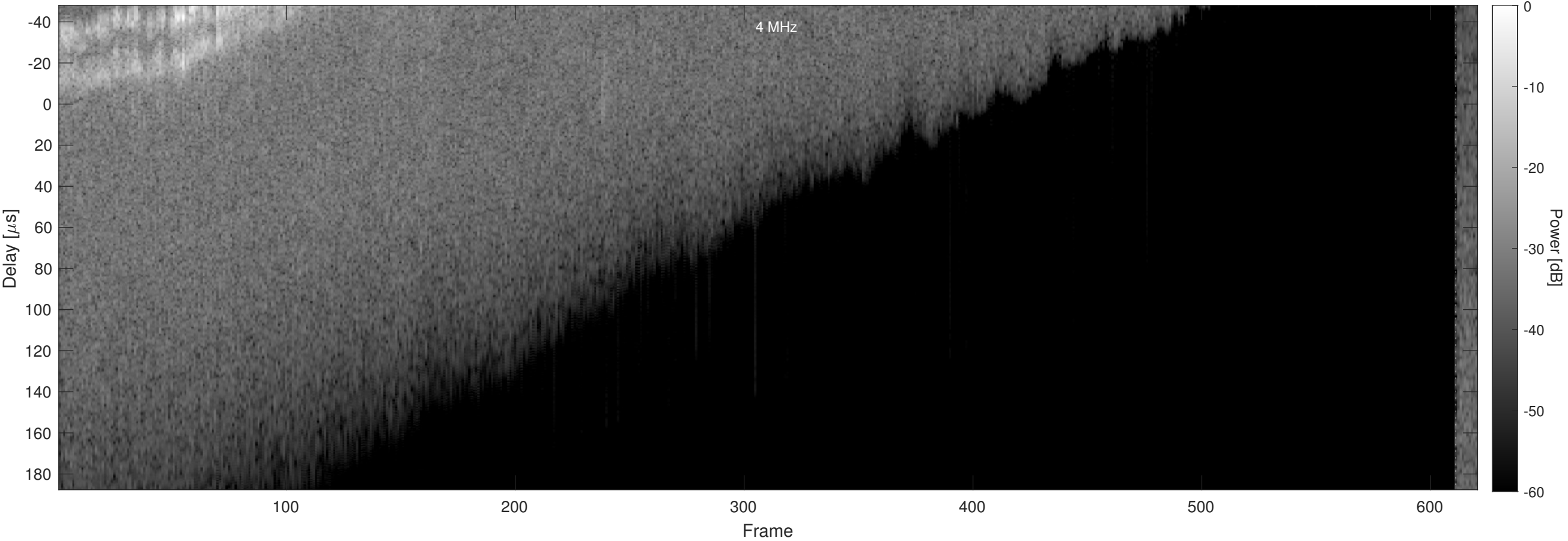
Orbit 7403, Chapman, Window, Channel 2
