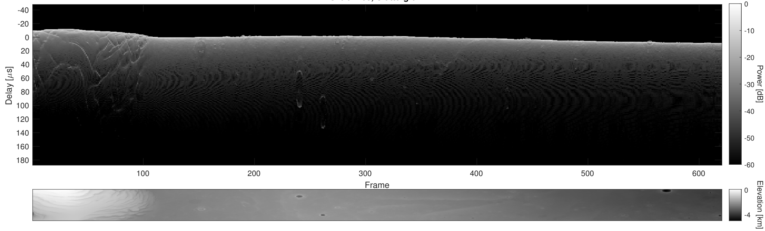
Orbit 7403, Cluttergram
