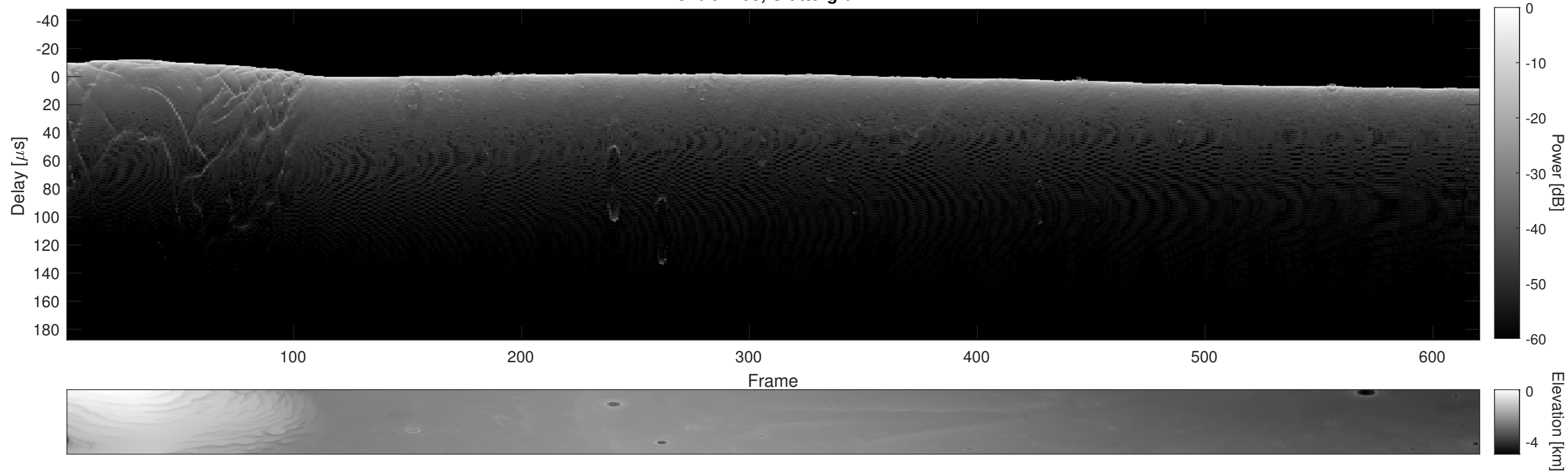
Orbit 7403, Cluttergram
