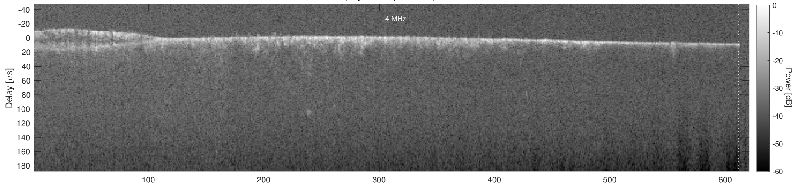
Orbit 7403, Cluttergram
