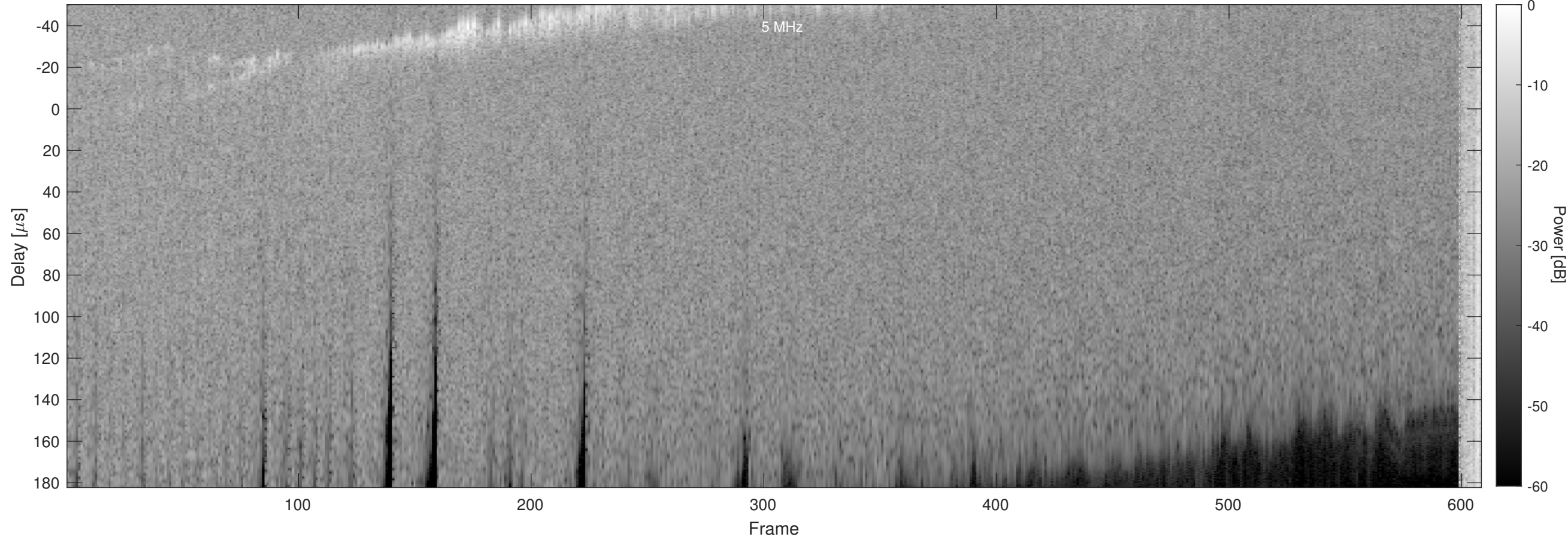
Orbit 7406, Chapman, No Window, Channel 2
