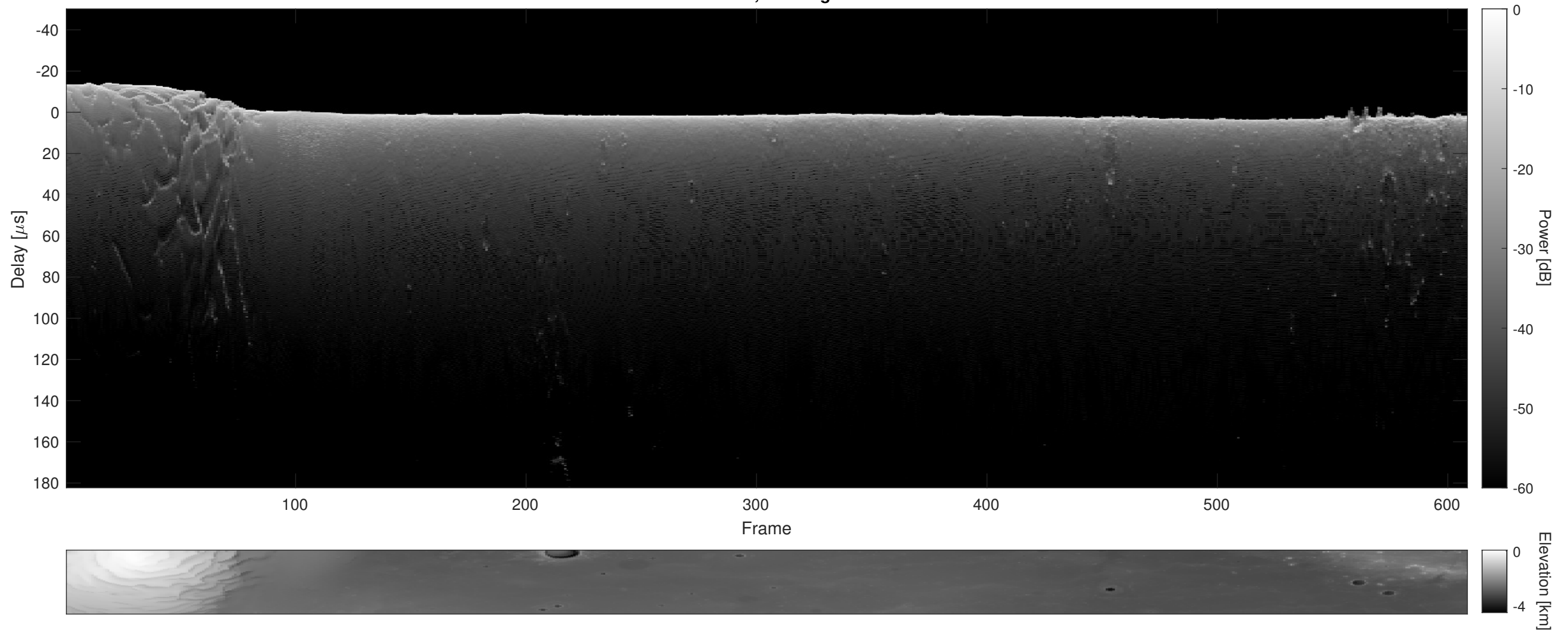
Orbit 7406, Cluttergram
