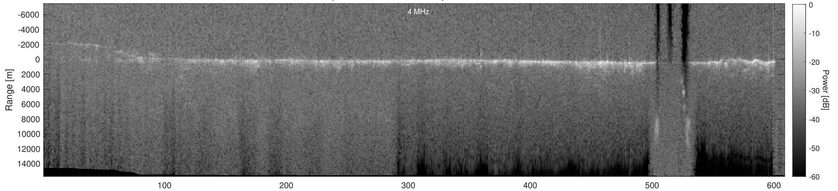
Orbit 7406, Depth-Corrected Cluttergram
