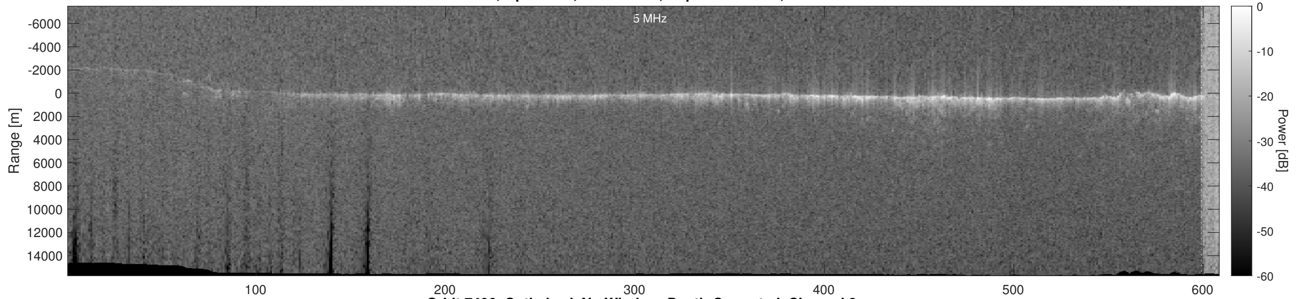
Orbit 7406, Optimized, No Window, Depth-Corrected, Channel 2
