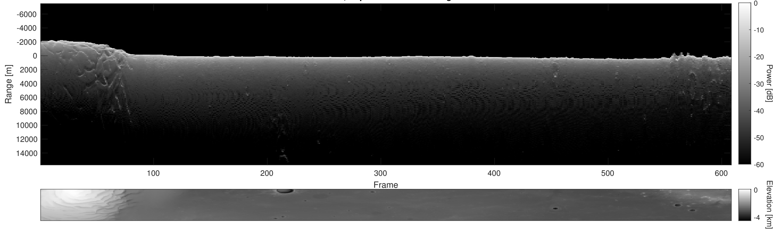
Orbit 7406, Depth-Corrected Cluttergram
