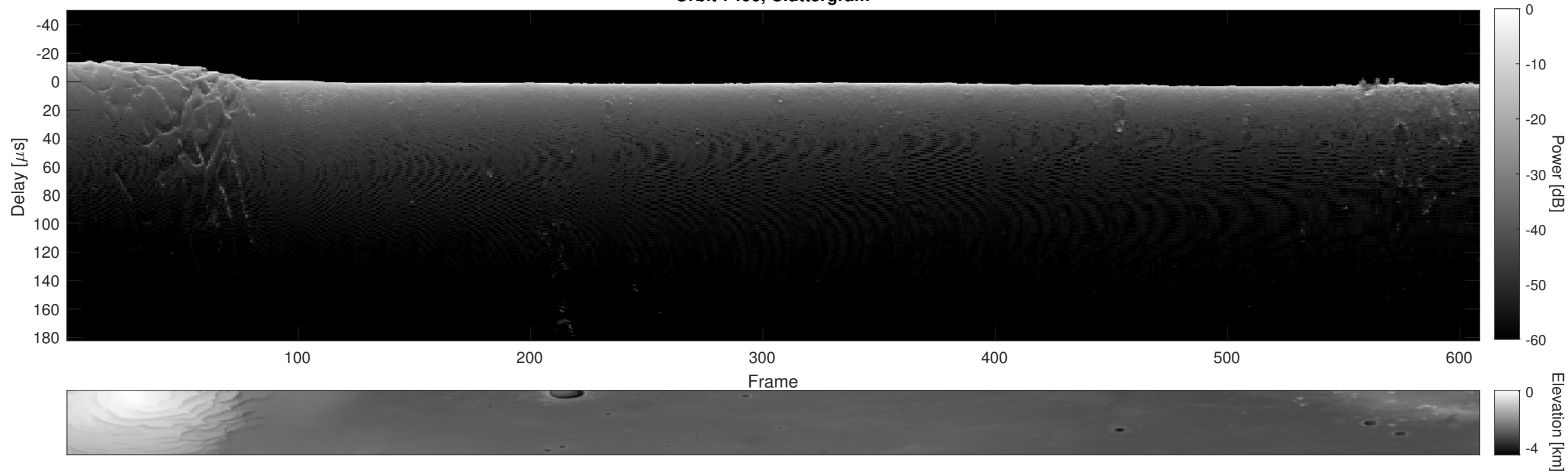
Orbit 7406, Cluttergram
