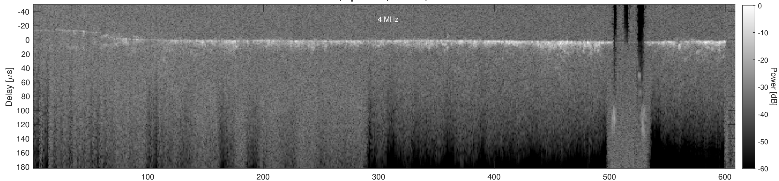
Orbit 7406, Cluttergram
