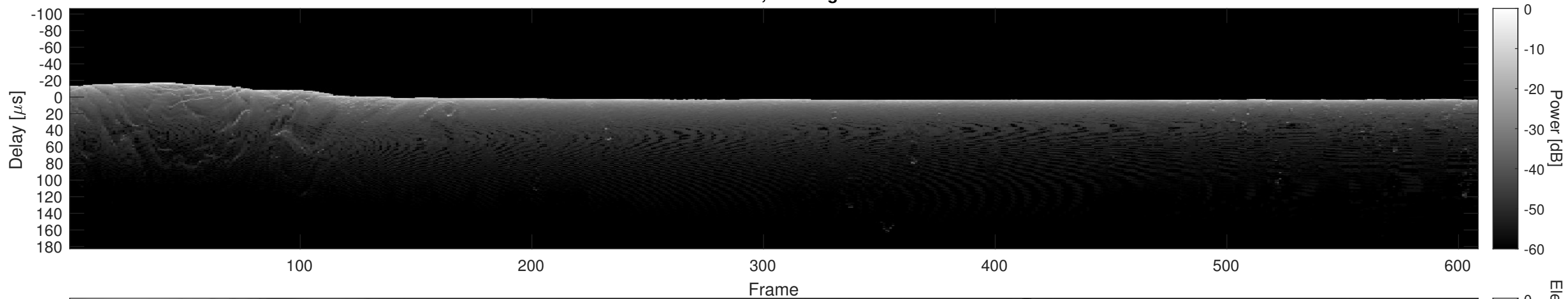
Orbit 7408, Cluttergram
