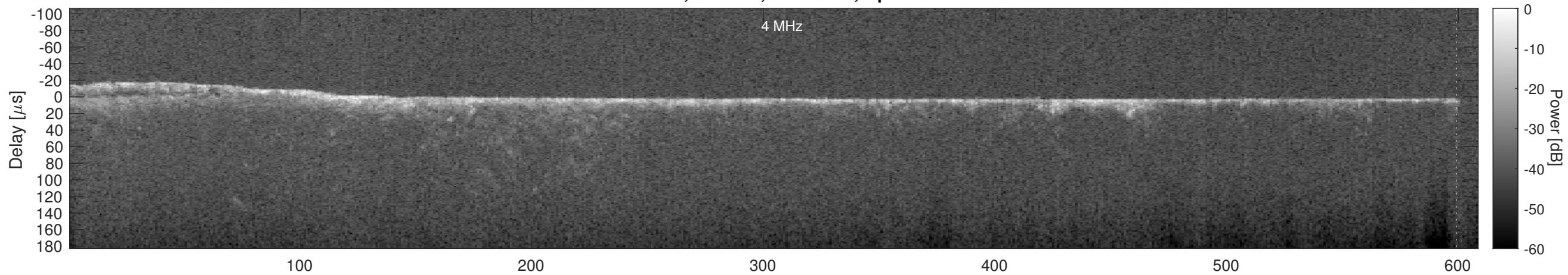
Orbit 7408, Cluttergram
