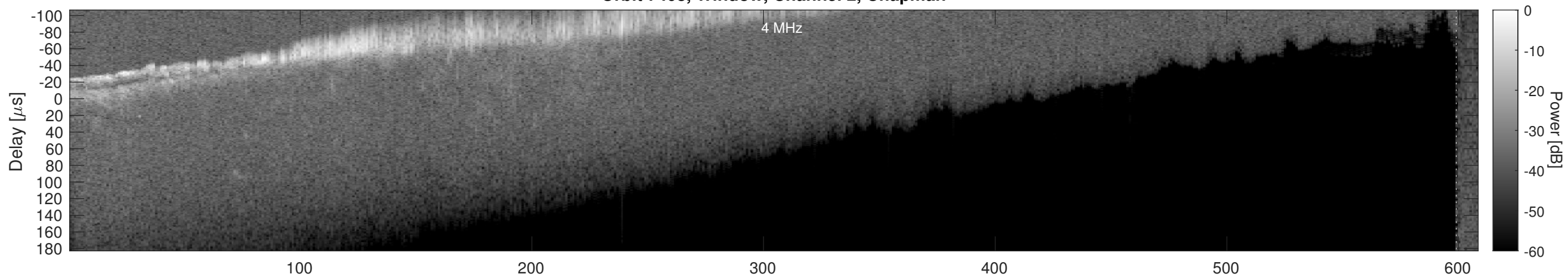
Orbit 7408, Window, Channel 2, Optimized
