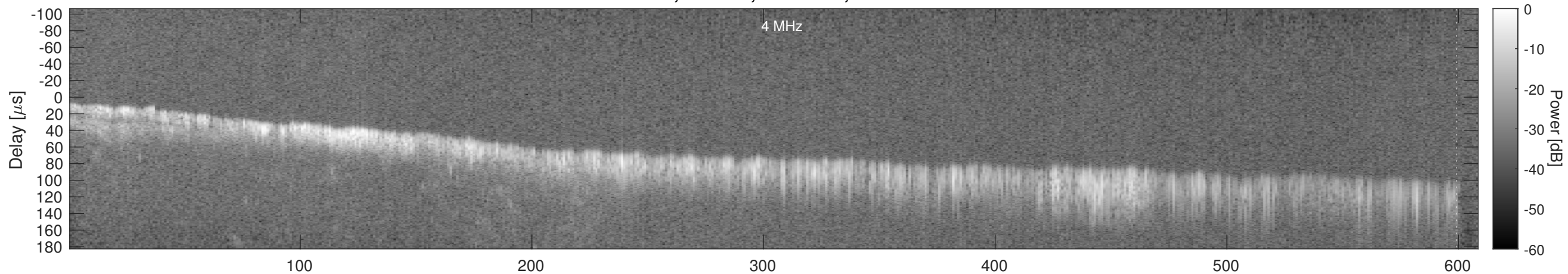
Orbit 7408, Window, Channel 2, Chapman
