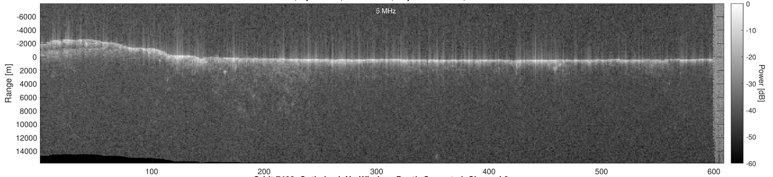
Orbit 7408, Optimized, No Window, Depth-Corrected, Channel 2
