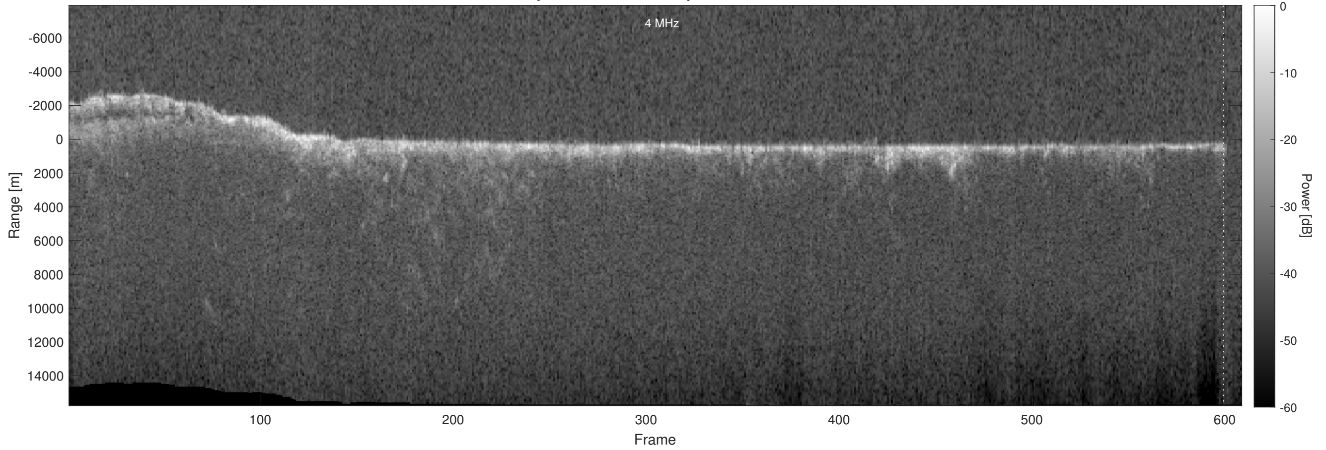
Orbit 7408, Optimized, Window, Depth-Corrected, Channel 2
