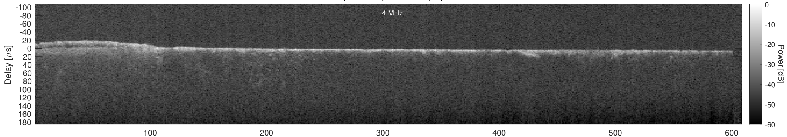
Orbit 7415, Cluttergram
