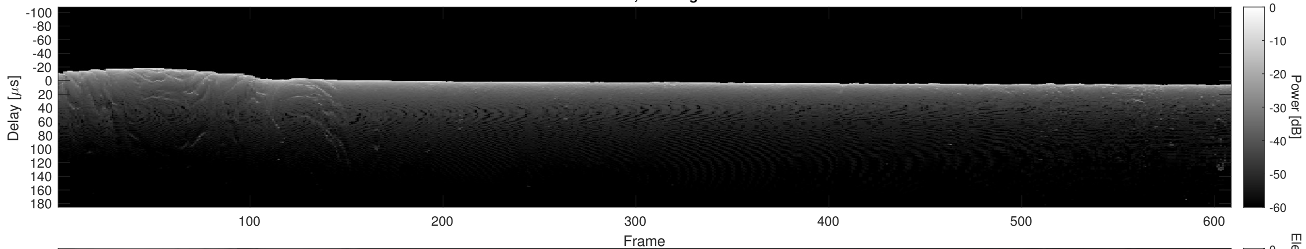
Orbit 7415, Cluttergram
