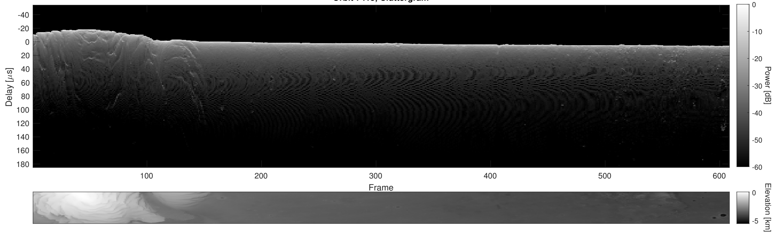
Orbit 7415, Cluttergram
