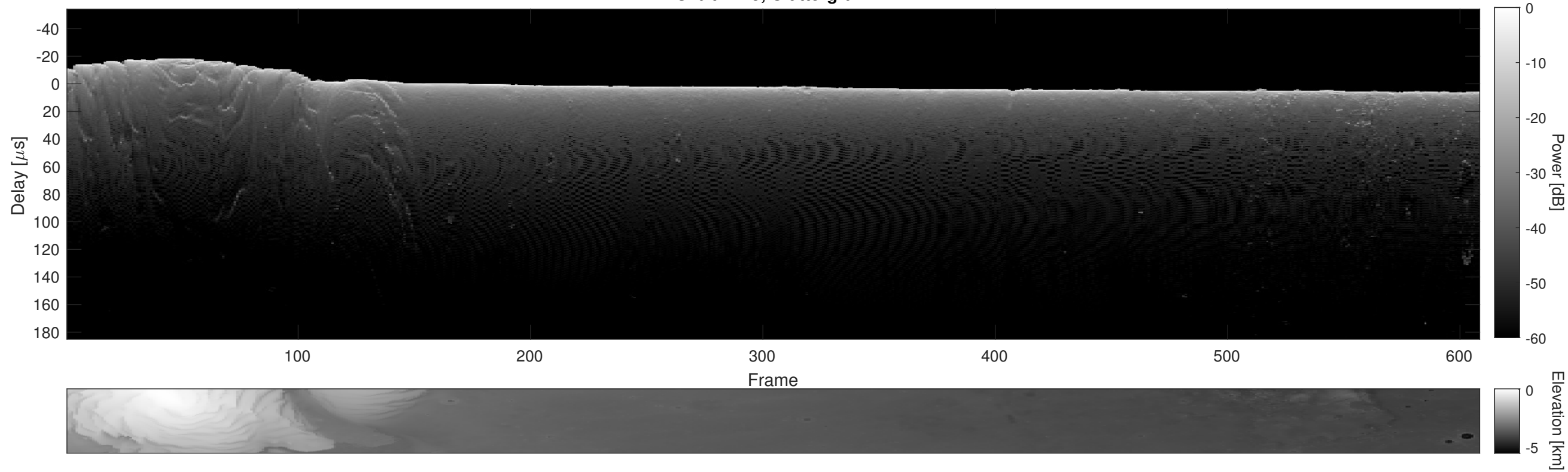
Orbit 7415, Cluttergram
