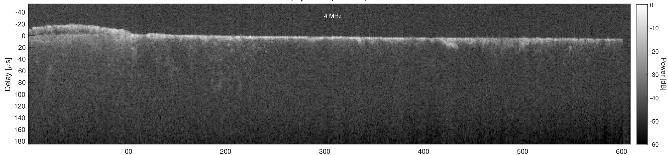
Orbit 7415, Cluttergram
