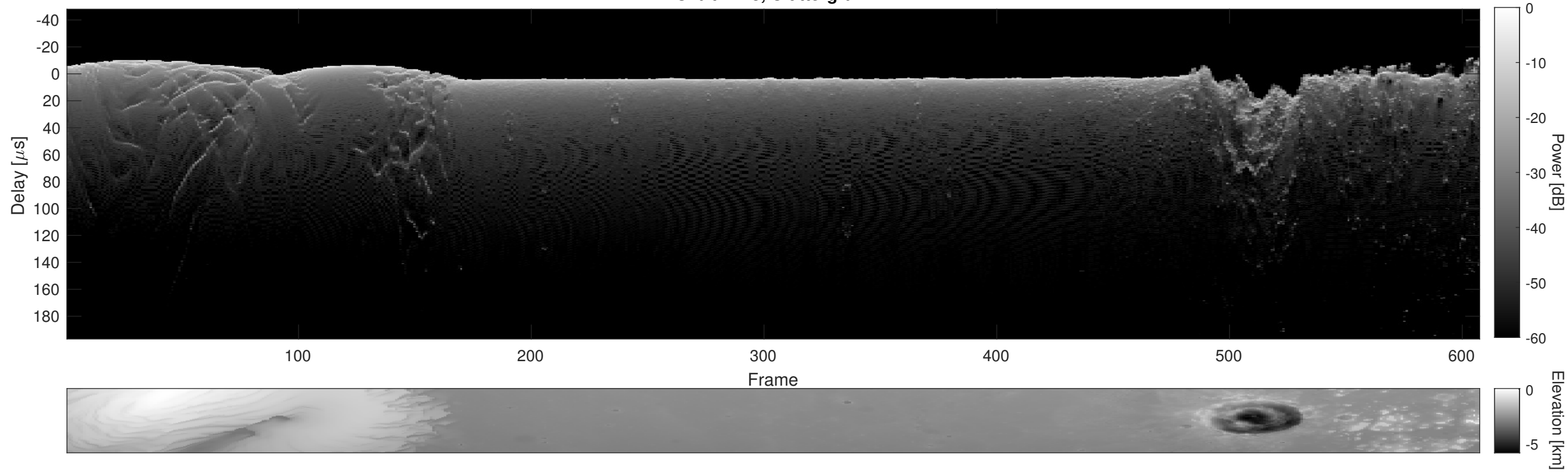
Orbit 7418, Cluttergram
