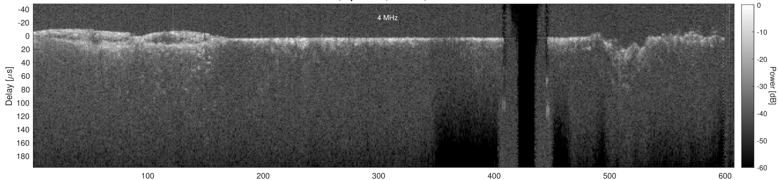
Orbit 7418, Cluttergram
