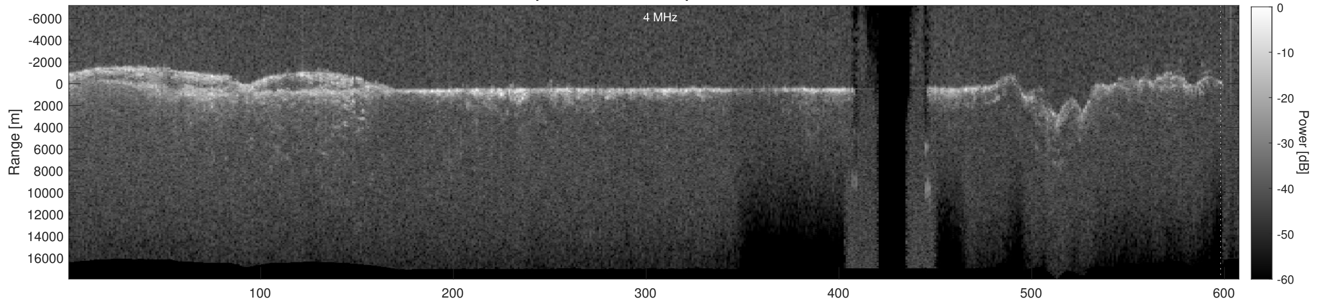
Orbit 7418, Depth-Corrected Cluttergram
