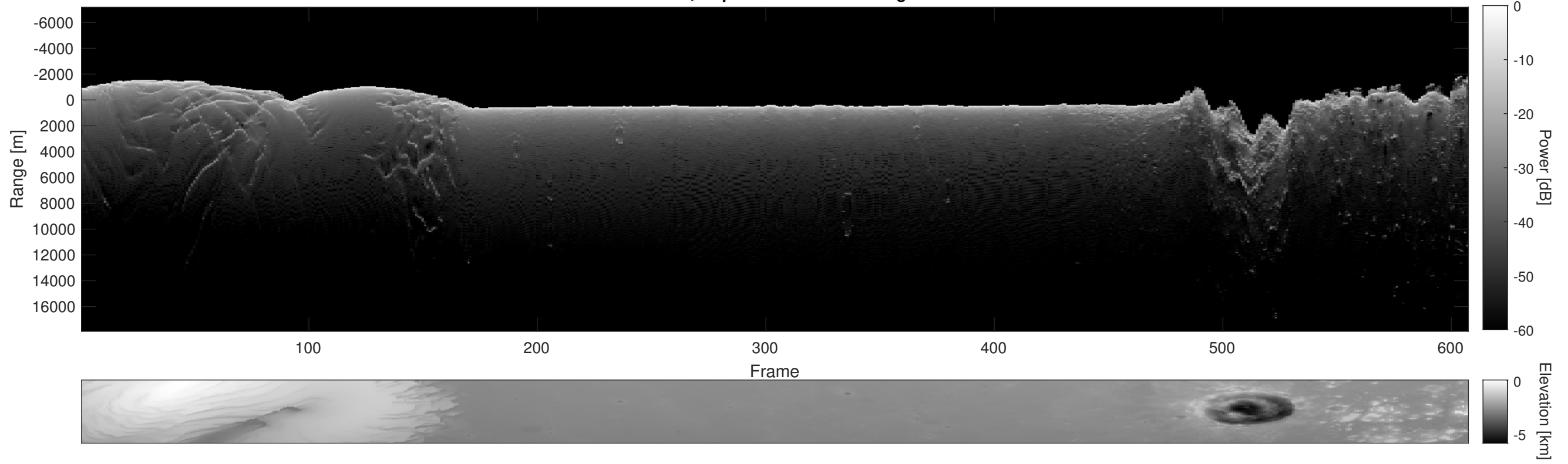
Orbit 7418, Depth-Corrected Cluttergram
