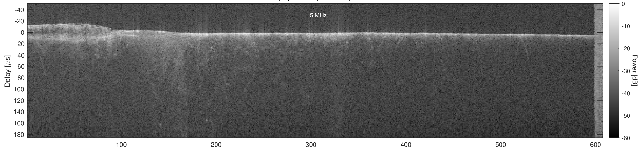
Orbit 7420, Optimized, Window, Channel 2
